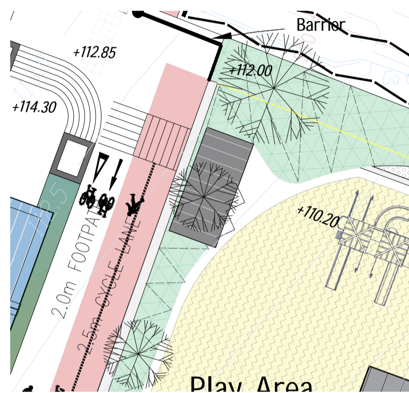
Childcare Building Site Location 1/200
