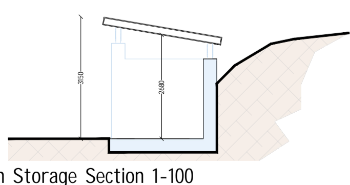
Bin Storage Section 1-100
