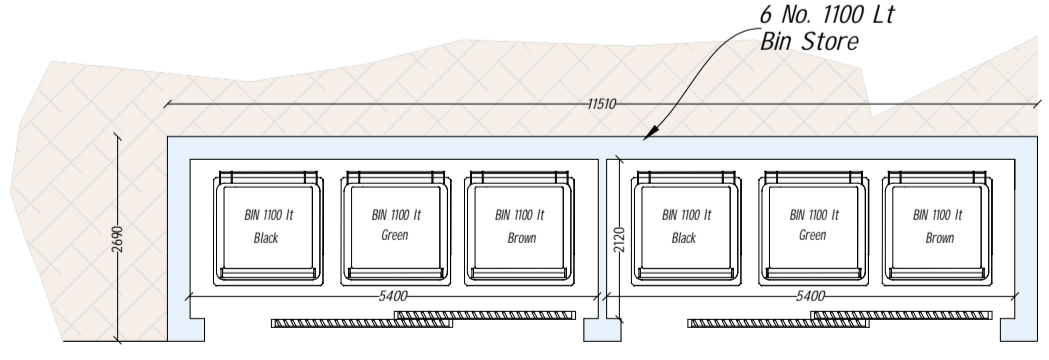
Bin Storage Plan 1-100
