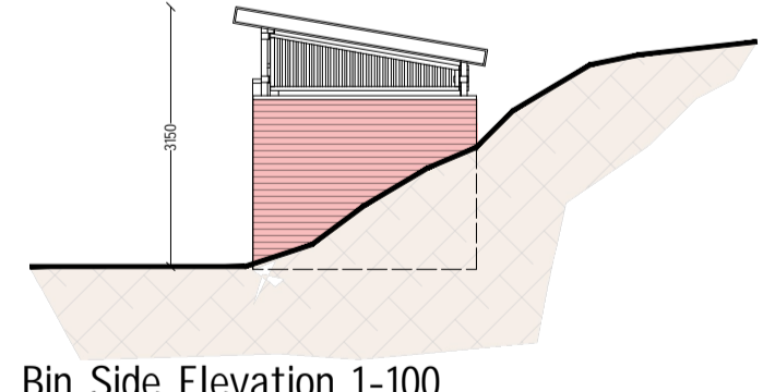
Bin Side Elevation 1-100
