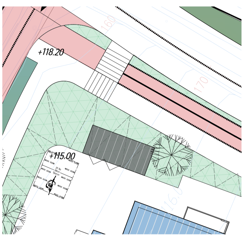
Exit Apartments (XAB) 248-257 Site Location 1/200
